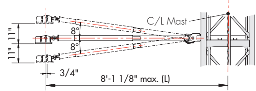
Inclination details
