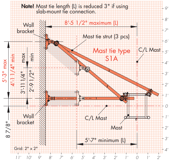
S1A Mast Tie Assembly Plan view
