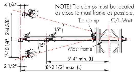
Inclination details
